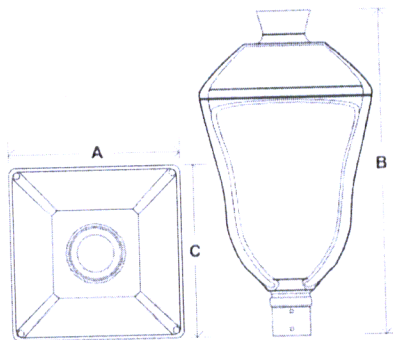
A x B x C (mm) – 373 x 705 x 373
